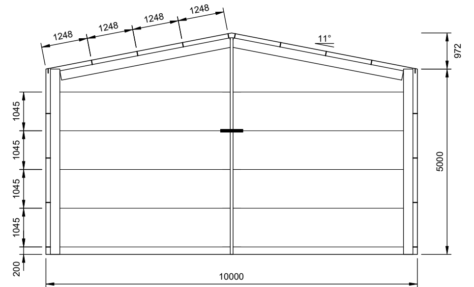
4 FRONT ELEVATION 3 SCALE: 1:100 FRAME #1
